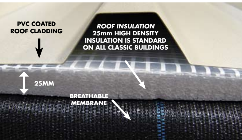
Shanette's Classic Roof Insulation System
