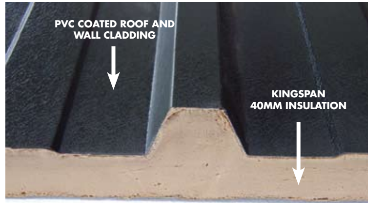
Shanette's Supreme Roof Insulation System
